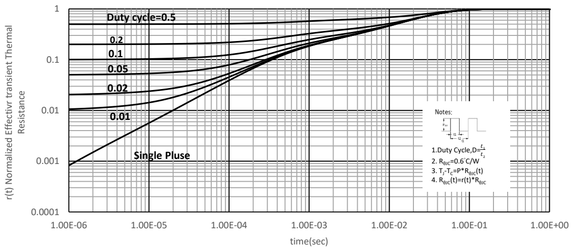
Fig.11. Effective Transient Thermal Impedance
