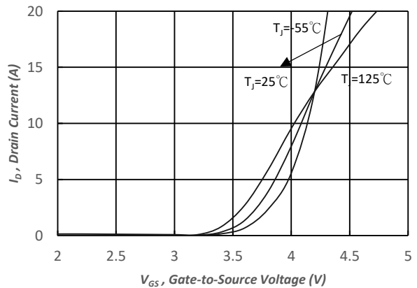
Fig.6 Transfer Characteristics
