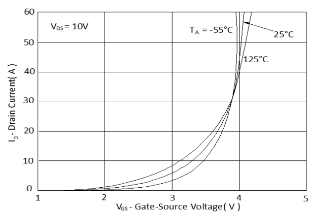
Fig.6 Transfer Characteristics
