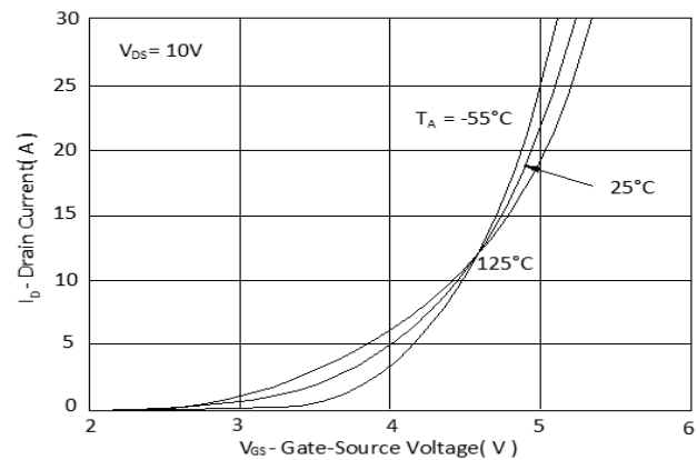
Fig.6 Transfer Characteristics
