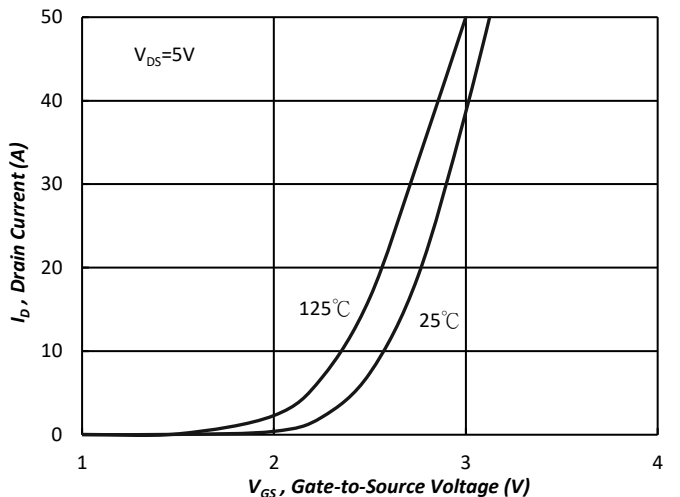
Fig.6 Transfer Characteristics
