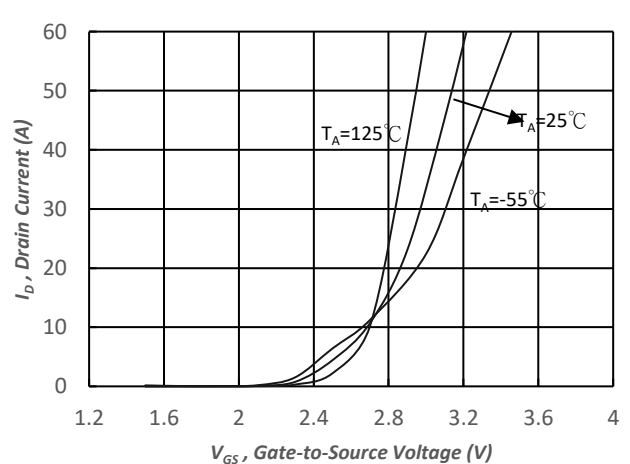
Fig.6 Transfer Characteristics
